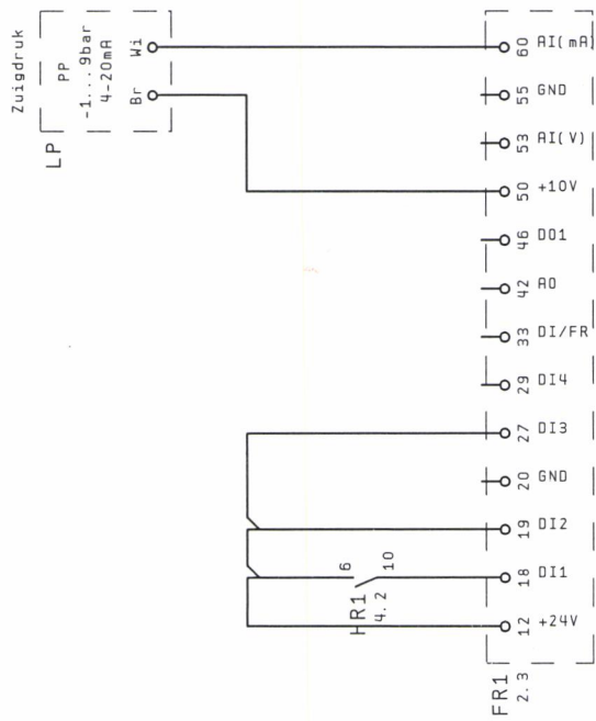
Frequentieregelaar 1 = Danfoss VLT2881 195N1123
